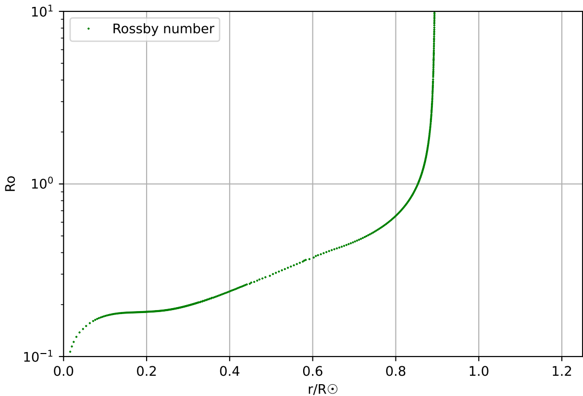
Rossby number, profile 129, age 2.67 \times 10^8
